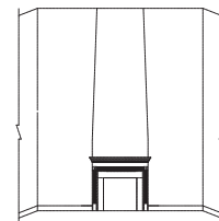
2 STORY SIDE WALL ELEVATION w/FIREPLACE
